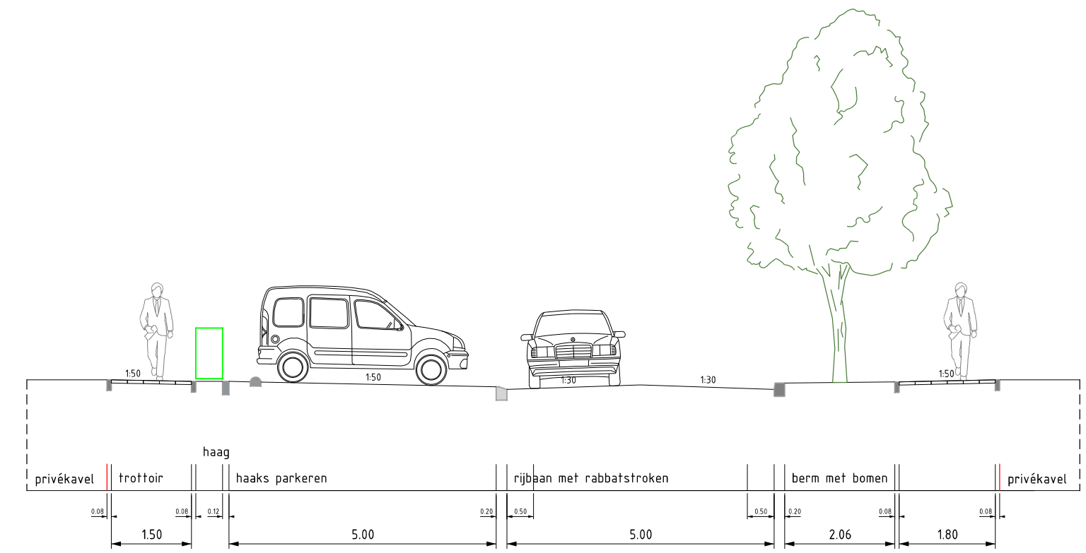
Principeprofiel A-A' (1:100)
